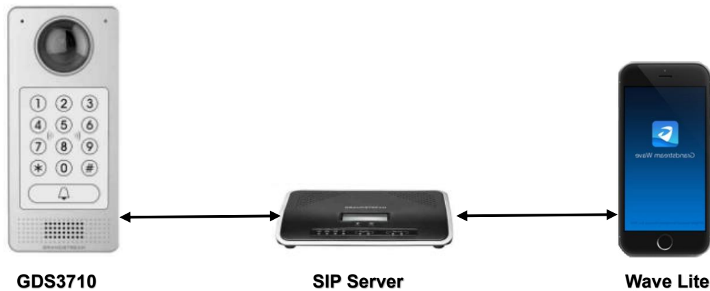
Figure 1 : Connecting GDS3710 with Wave Lite
